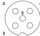
FEMALE SOCKET
